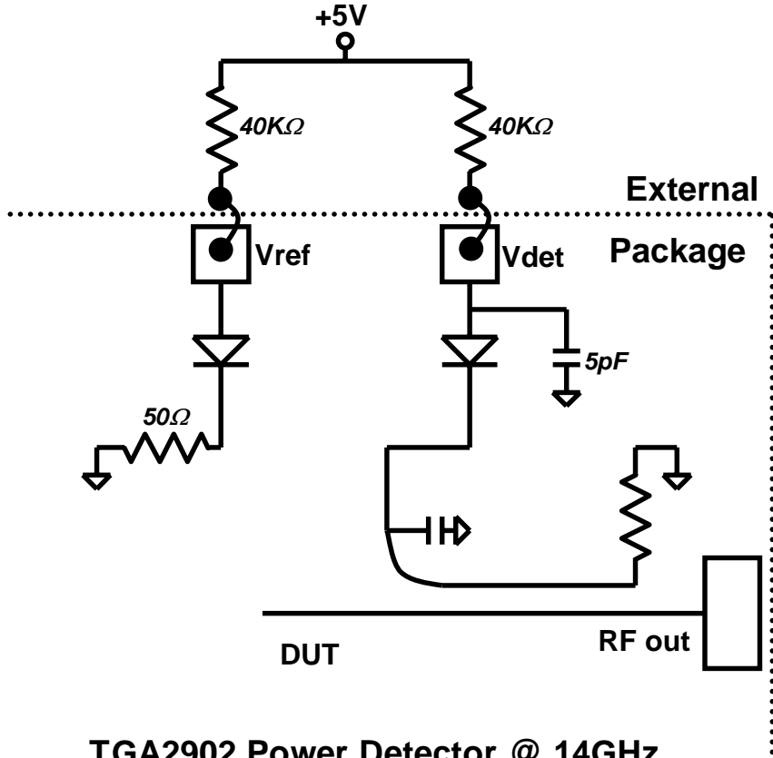
TGA2902 Power Detector @ 14GHz
