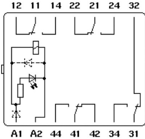
Circuit diagram
