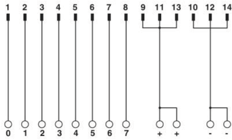
VIP-2/SC/FLK14/PLC connection scheme
