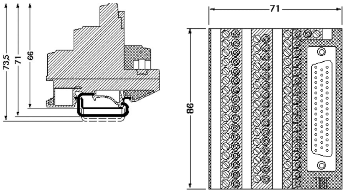
Dimensioned drawing
