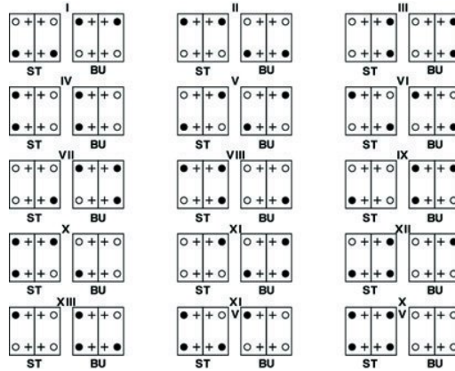
Coding for housings with two contact inserts
