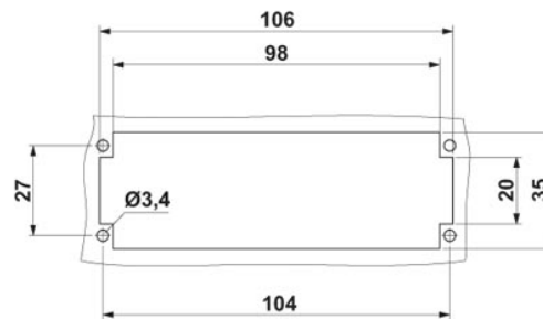
Panel cutout
