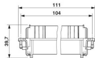
Female insert
