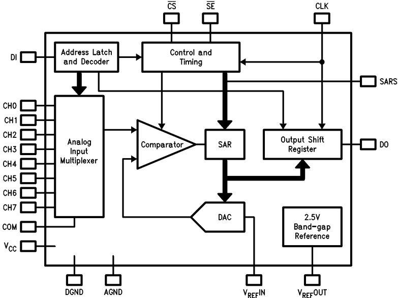
ADC08138 Simplified Block Diagram
