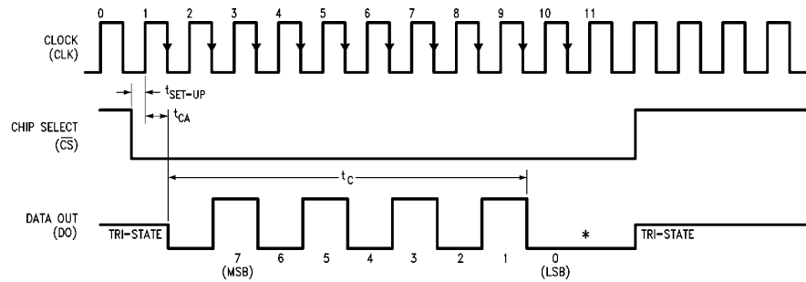
ADC08131 Timing
