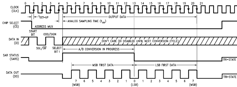
ADC08134 Timing
