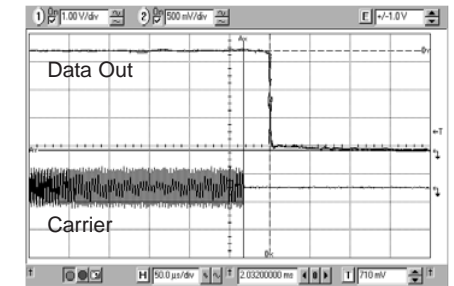
Figure 6: Typical Receiver Turn-Off Time
