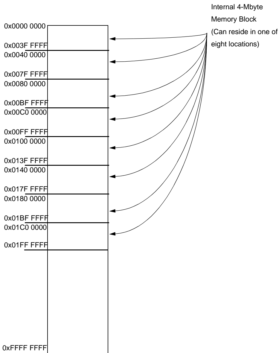
Figure 3. MPC561/MPC563 Memory Map
