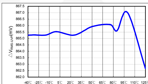
Figure 34. \Delta V_{RMS-UVF} vs. Temperature
