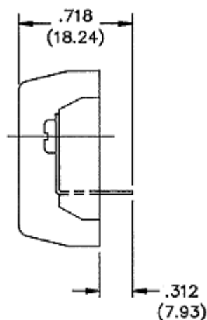
"Y" Terminals
