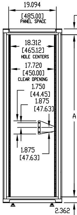
FRONT VIEW (LESS DOOR)
