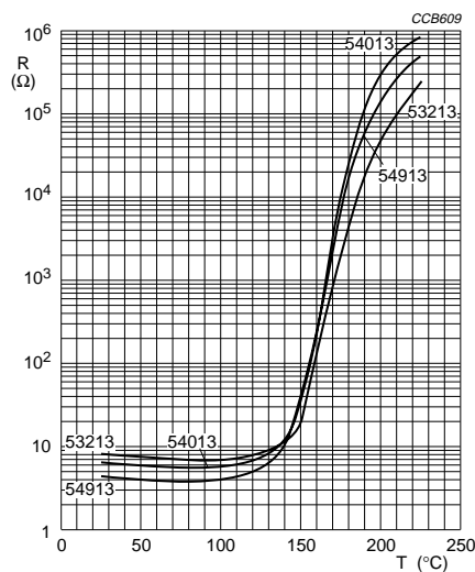
Fig.23 Typical resistance/temperature characteristic for 2322 662 53213 and 663 54013/54913.
