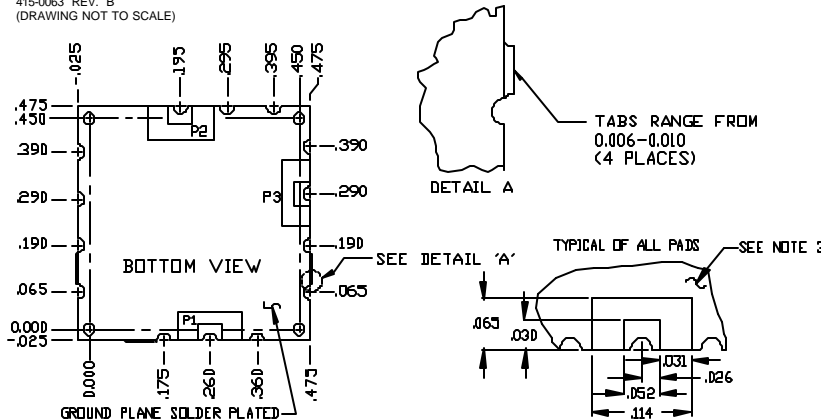
PHYSICAL DIMENSIONS
