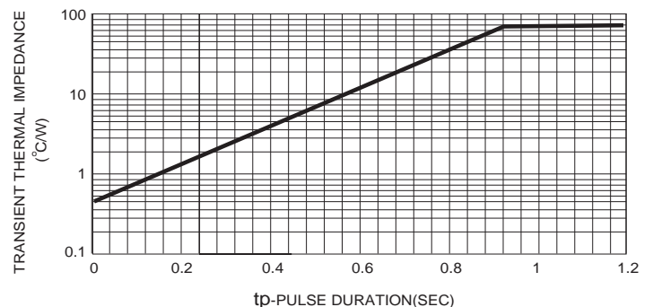
FIG.8 - TYP. TRANSIENT THERMAL IMPEDANCE
