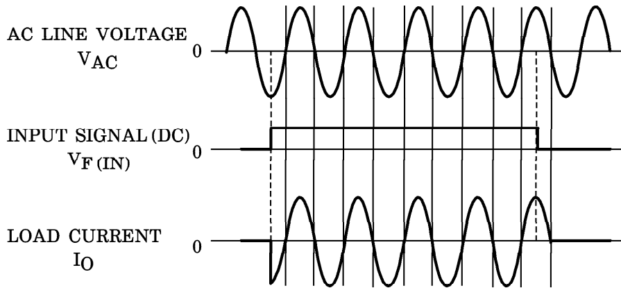
Fig. 1. SWITCHING WAVEFORM
