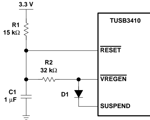
Figure 13–2. External Circuit
