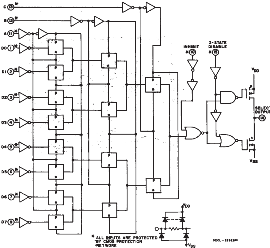
Fig. 1 - Logic diagram.
