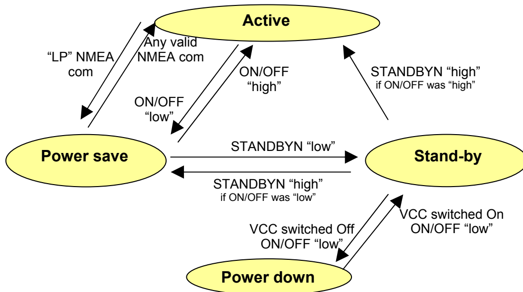
Figure 1 Switching between operating modes
