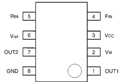
Fig.1 Pin assignments
