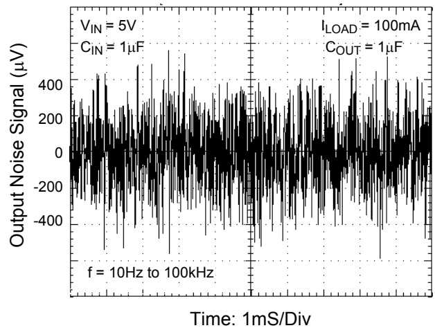
Output Noise
