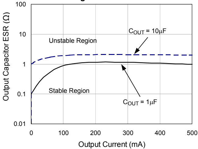
Range of Stable ESR
