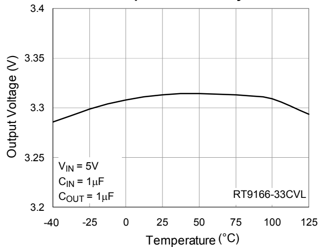
Temperature Stability
