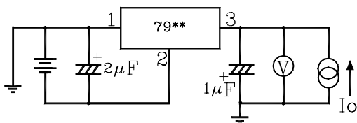
TEST CIRCUIT 1
