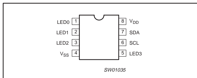
Figure 1. Pin configuration
