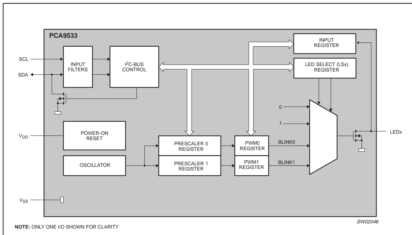
Figure 2. Block diagram
