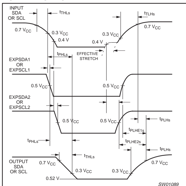
Waveform 1.
