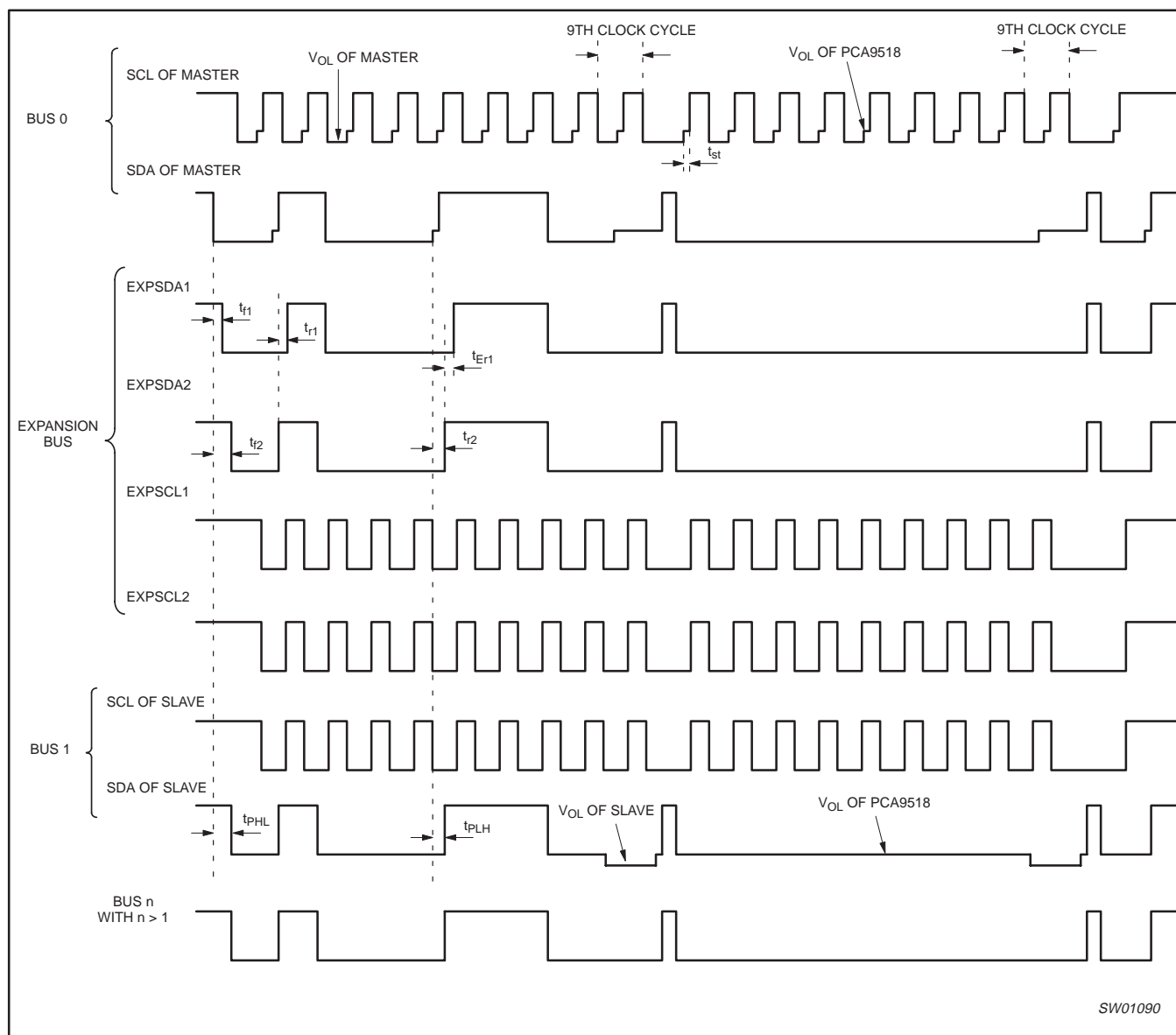
Figure 5. Bus waveforms
