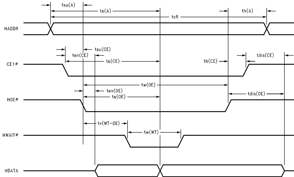
FIGURE 1. Attribute Memory Read Timing
