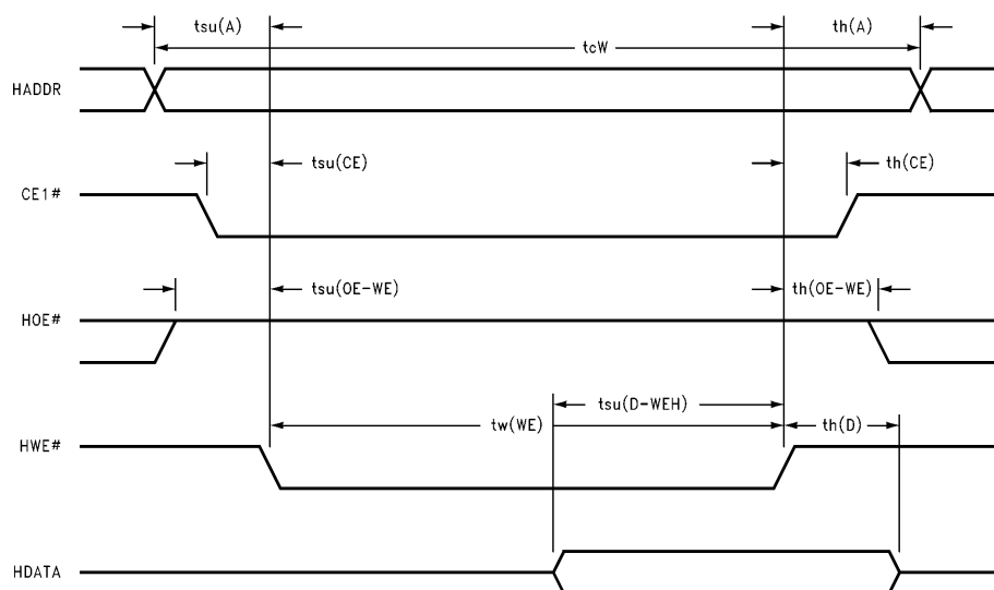
FIGURE 2. Attribute Memory Write Cycle Attribute Memory Write Cycle Specifications (See Figure 2)
