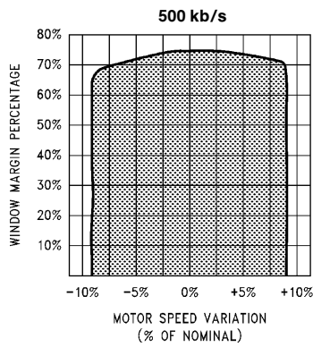
FIGURE 5-3. PC8477B Dynamic Window Margin Performance
