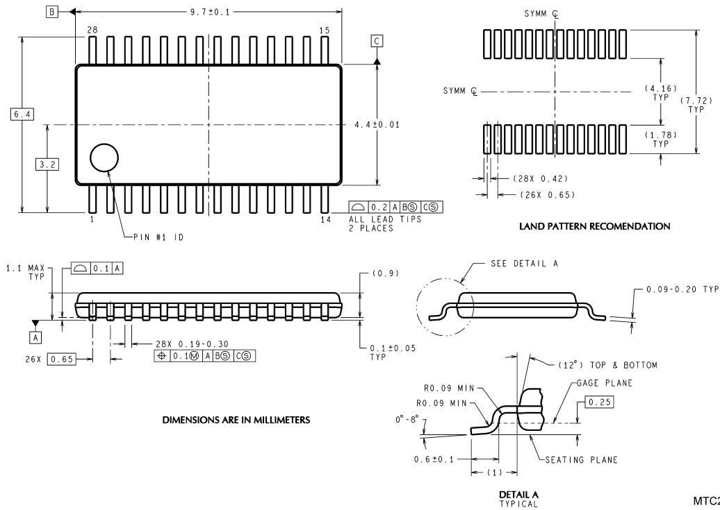
28-Lead TSSOP Package NS Package Number MTC28
