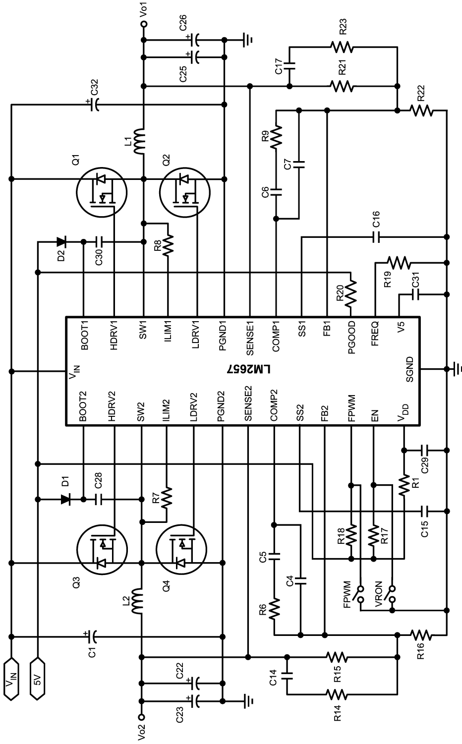
FIGURE 13. Typical Application (Expanded View)
