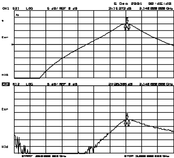
S21 & S12 Condition V_{LNA}=2.85V V_{MIX}=V_{LO}=0V
