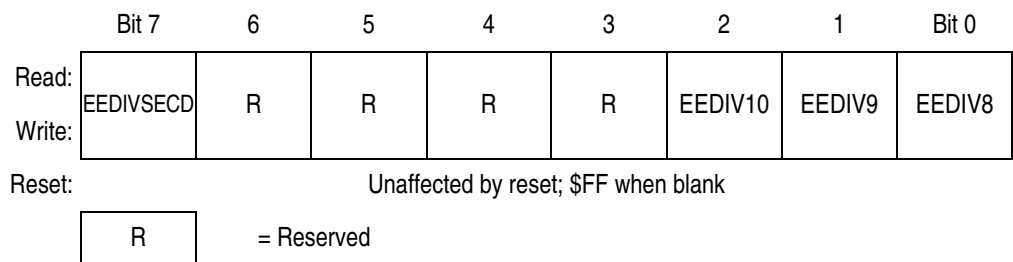
Figure 7-7. EEPROM-2 Divider Non-Volatile Register High (EE2DIVHNVR)
