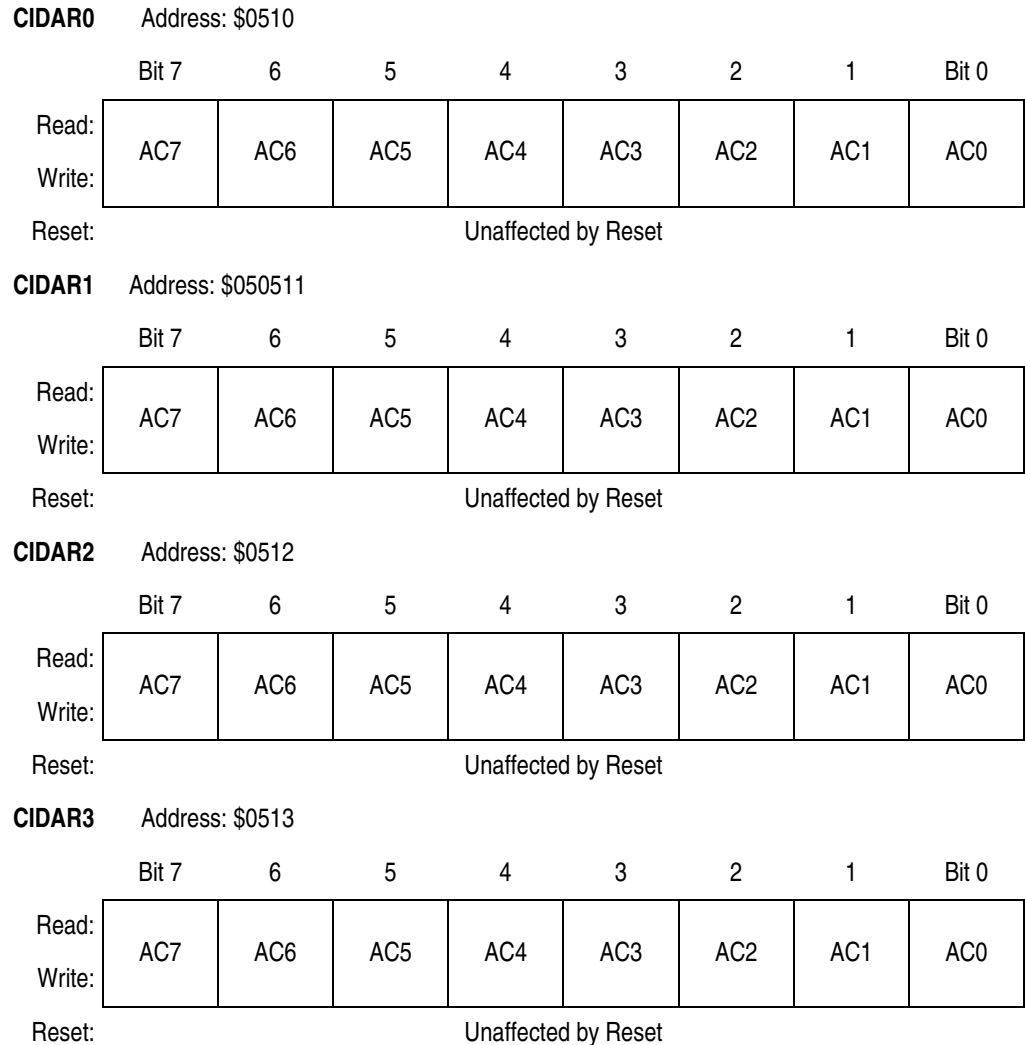
Figure 23-26. Identifier Acceptance Registers (CIDAR0–CIDAR3)
