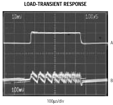
CIRCUIT OF FIGURE 2 V_+ = 6\text{V} , V_{OUT} = -5\text{V} A: I_{LOAD} , 30mA TO 1A, 1A/div B: V_{OUT} , 100mV/div, AC-COUPLED
