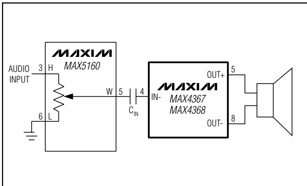
Figure 8. MAX4367/MAX5160 Volume Control Circuit
