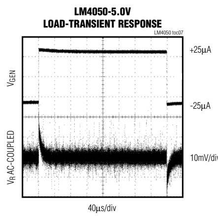
I_{SHUNT} = 100\mu\text{A} \pm 25\mu\text{A} R_L = 100\text{k}\Omega , SEE FIGURE 1.
