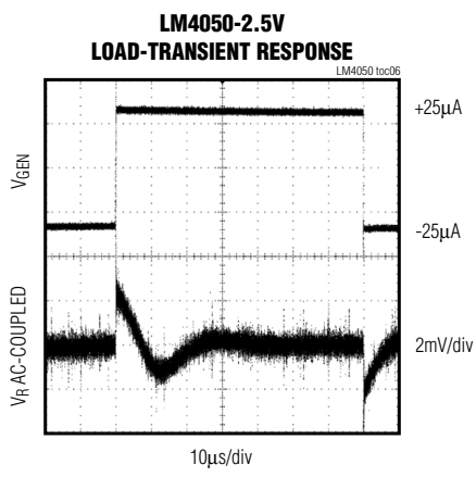
CH1: V_{GEN} 2V/div CH2: V_R AC-COUPLED 2mV/div I_{SHUNT} = 100\mu\text{A} \pm 25\mu\text{A} , R_L = 100\text{k}\Omega , SEE FIGURE 1.
