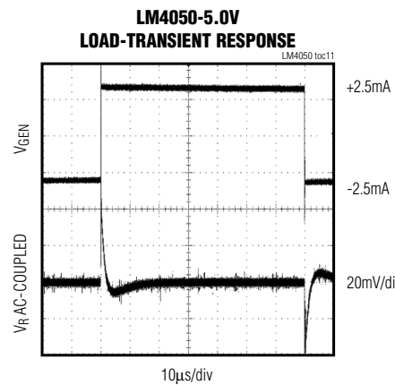
I_{SHUNT} = 10\text{mA} \pm 2.5\text{mA} R_L = 1\text{k}\Omega , SEE FIGURE 1.
