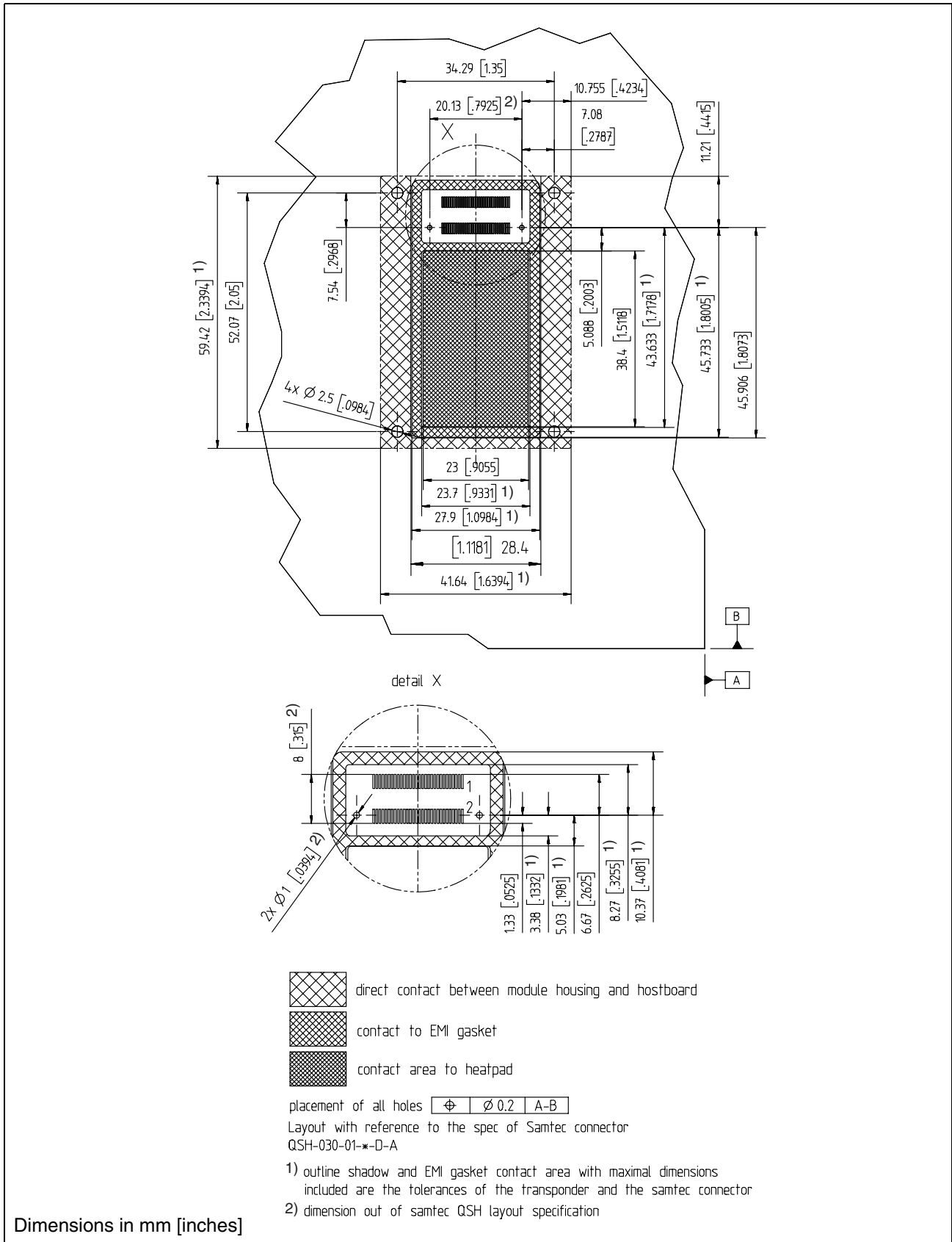
Figure 12 Hostboard Contact Area
