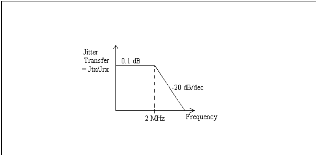
Figure 2 Sonet Jitter Transfer Mask (ITU-T G.958 & Bellcore GR-253)
