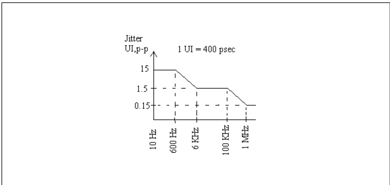
Figure 3 Sonet Jitter Tolerance Mask (Bellcore GR-253)
