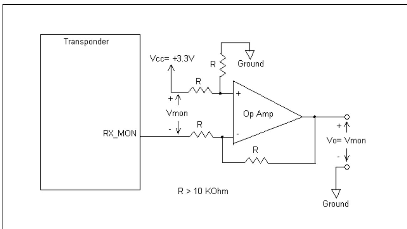
Figure 11 Conversion of Rx_MON Output to a Voltage with Respect to Ground
