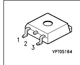
P-TO263-3-2
