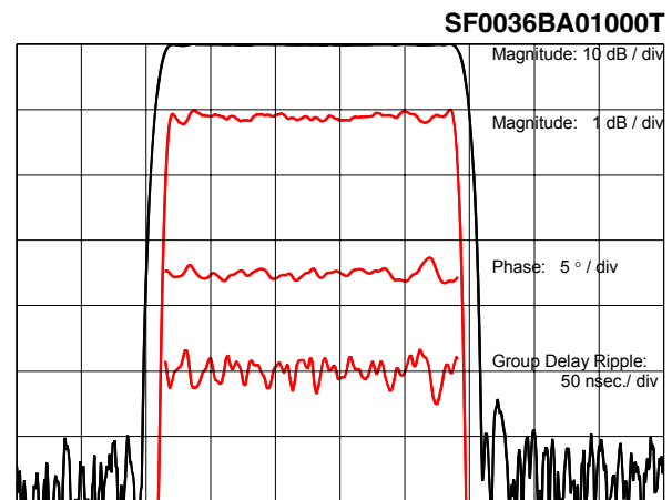
Frequency: 1.5 MHz/div
