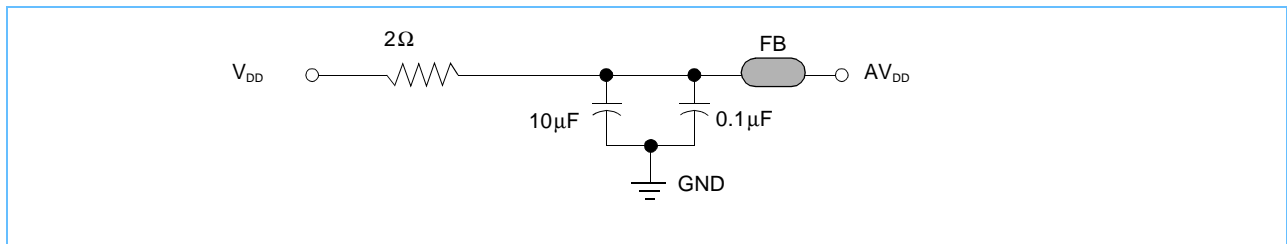
Figure 6-1. PLL Power Supply Filter Circuit
