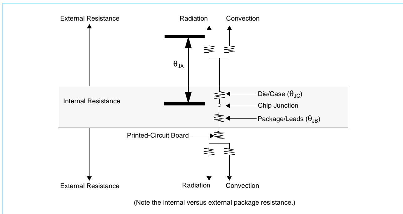
Figure 6-4. PBGA Package Thermal Model
