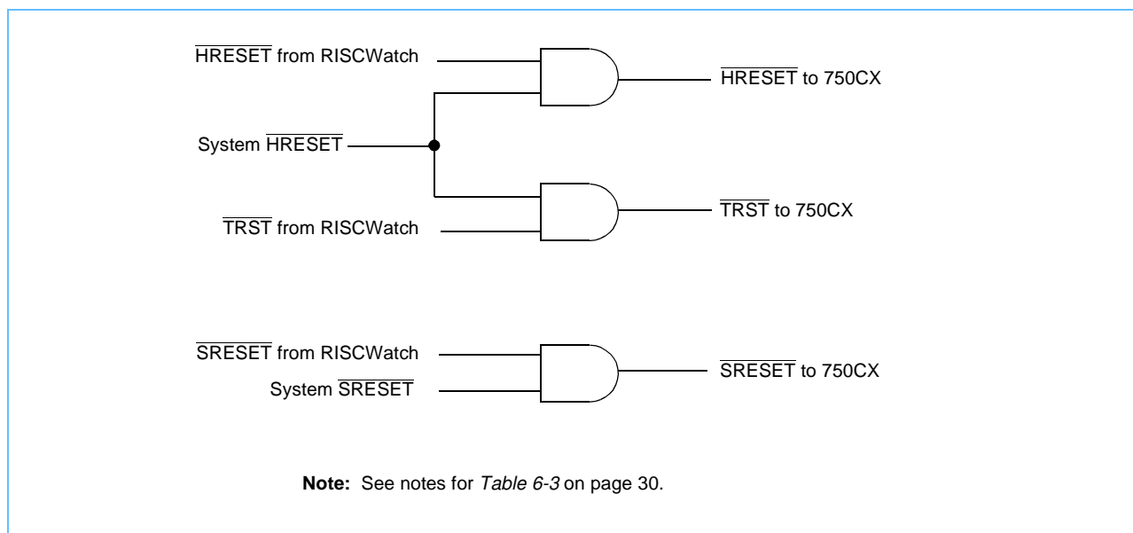
Figure 6-3. IBM RISCWatch JTAG to \overline{HRESET} , \overline{TRST} , and \overline{SRESET} Signal Connector
