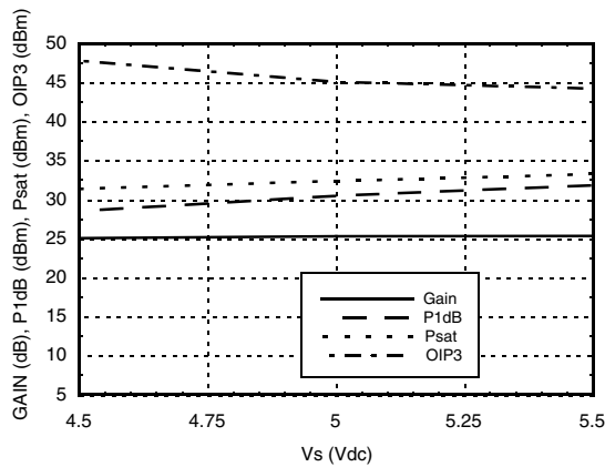
Gain, Power & IP3 vs. Supply Voltage @ 2100 MHz
