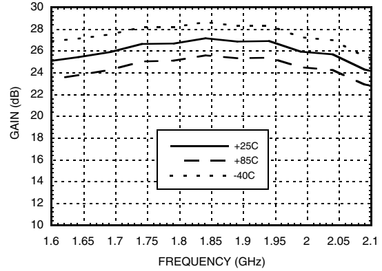
Gain vs. Temperature @ 1900 MHz
