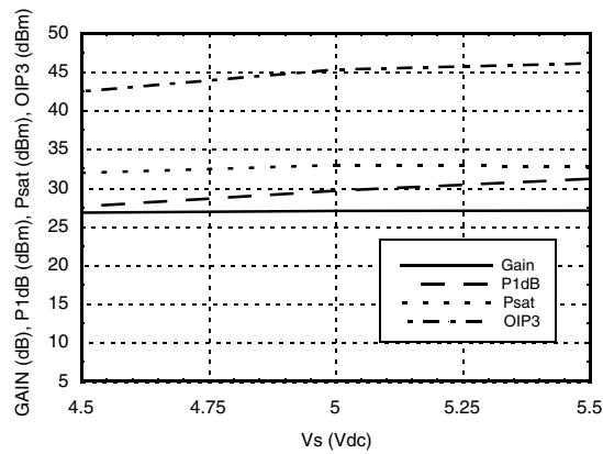
Gain, Power & IP3 vs. Supply Voltage @ 1900 MHz
