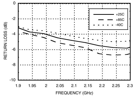
Output Return Loss vs. Temperature @ 2100 MHz
