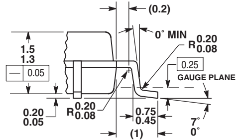
VIEW AA
