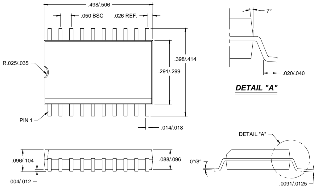
Figure 15. 20-Pin SOIC Package Outline
