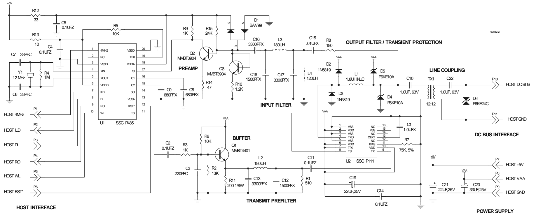
Figure 14. P485 Reference Application
