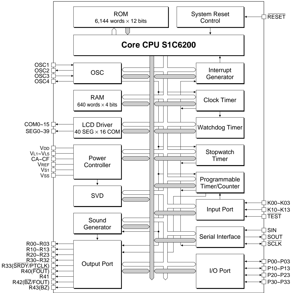
Fig. 1.2.1 Block diagram
