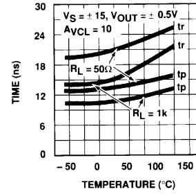
Rise Time and Prop Delay vs Temperature
