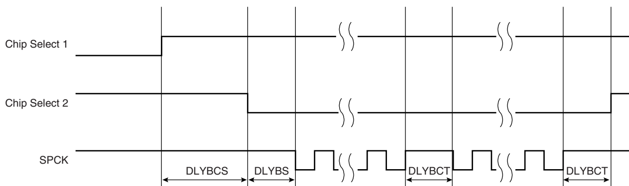
Figure 29-7. Programmable Delays
