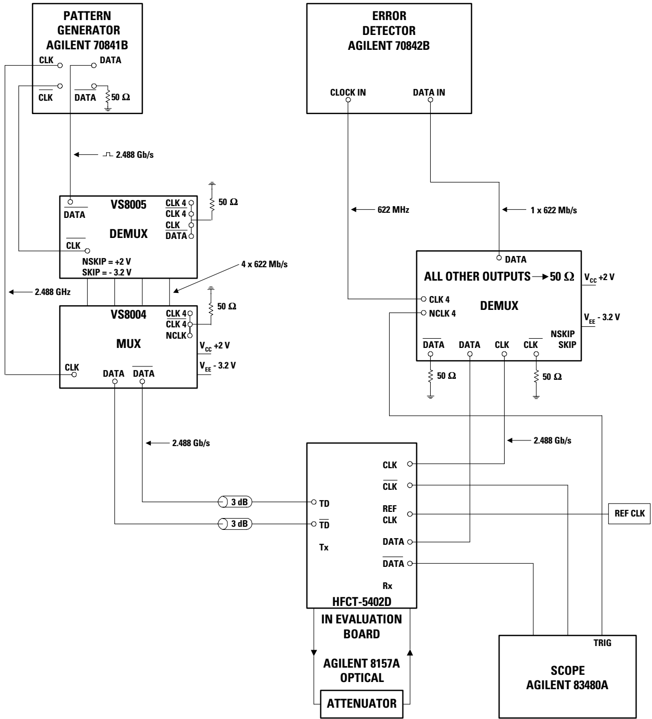
Figure 21. Test Configuration
