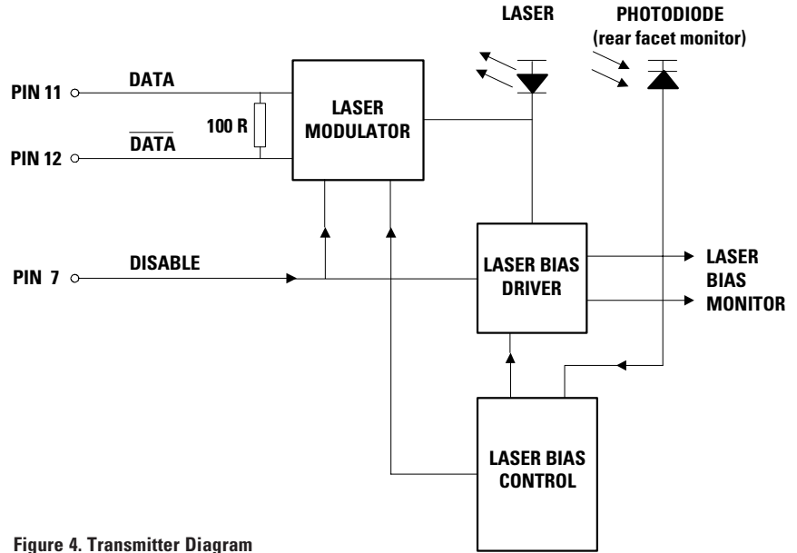
Figure 4. Transmitter Diagram
