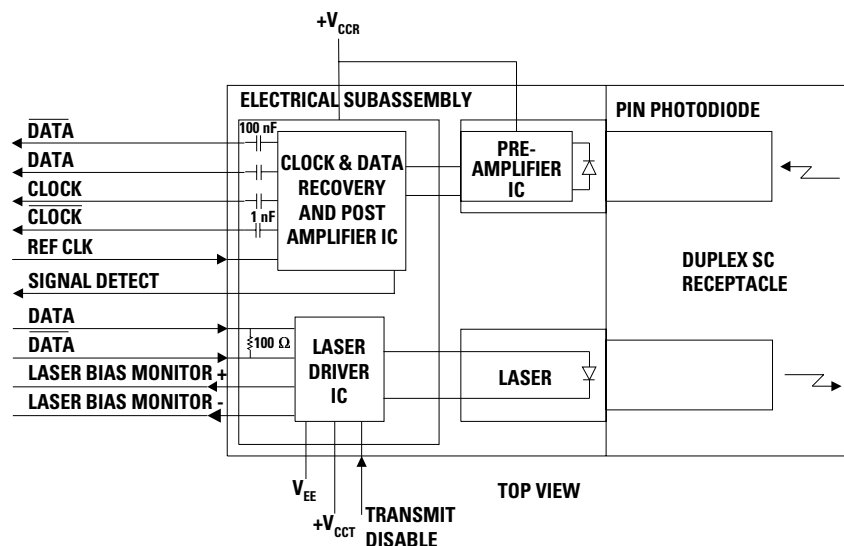
Figure 1. Block Diagram
