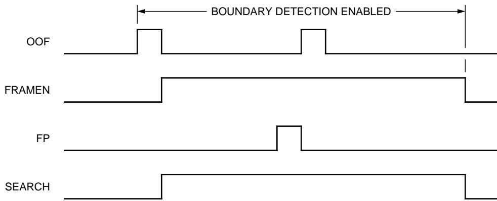
Figure 14. FRAMEN Timing
