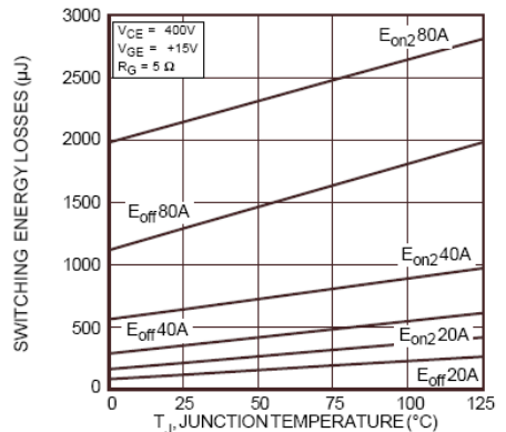
FIGURE 16, Switching Energy Losses vs Junction Temperature
