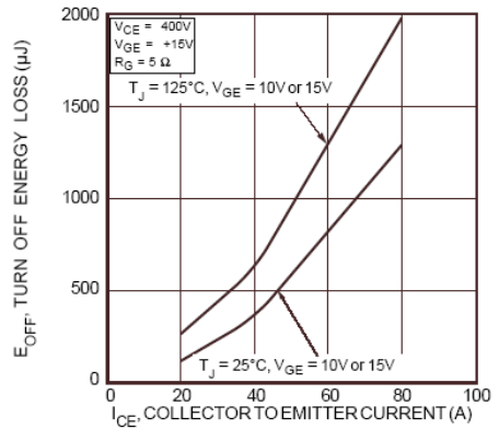
FIGURE 14, Turn Off Energy Loss vs Collector Current
