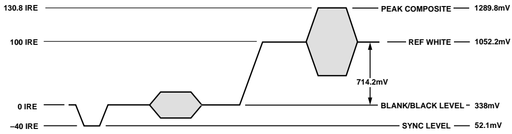
Figure 48. NTSC Composite Video Levels
