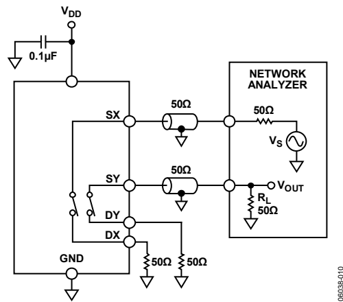
Figure 29. Channel-to-Channel Crosstalk
