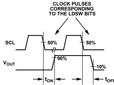
Figure 25. Switching Times
