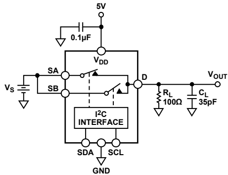
Figure 26. Break-Before-Make Time Delay
