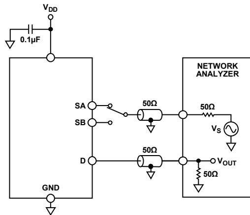
Figure 27. Bandwidth
