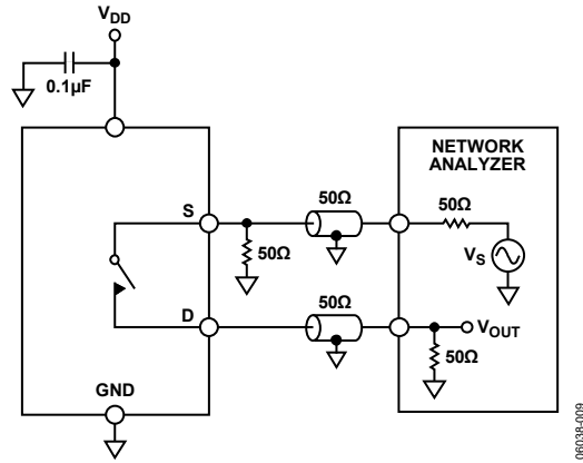
Figure 28. Off Isolation
