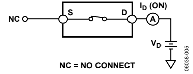
Figure 24. On Leakage
