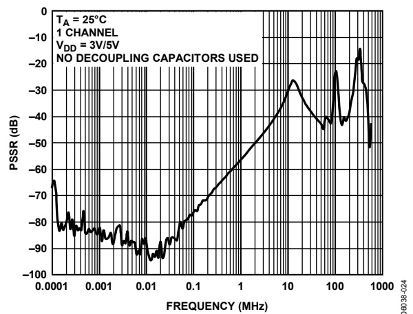
Figure 16. PSSR vs. Frequency
