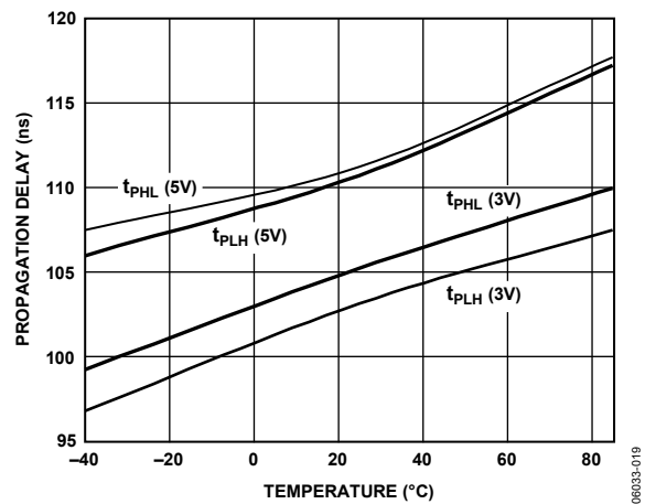
Figure 19. I^2C to GPO Propagation Delay vs. Temperature (ADG799G Only)
