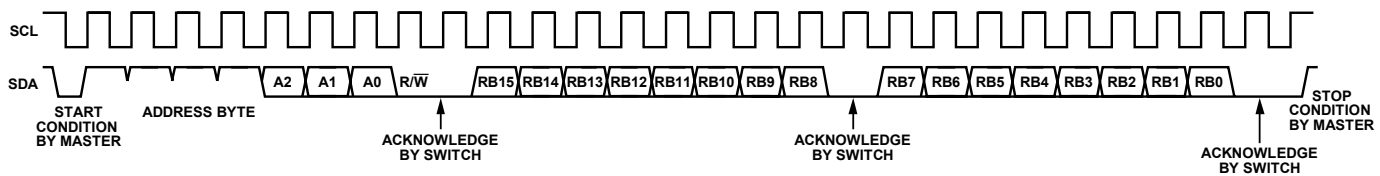
Figure 32. ADG799A/ADG799G Read Operation
