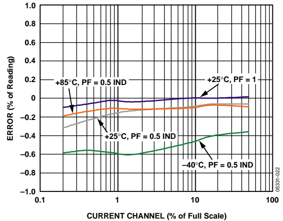
Figure 8. Error as a % of Reading over Temperature with External Reference (PF = 0.5)
