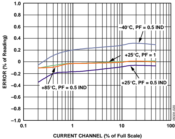
Figure 6. Error as a % of Reading over Temperature with On-Chip Reference (PF = 0.5)
