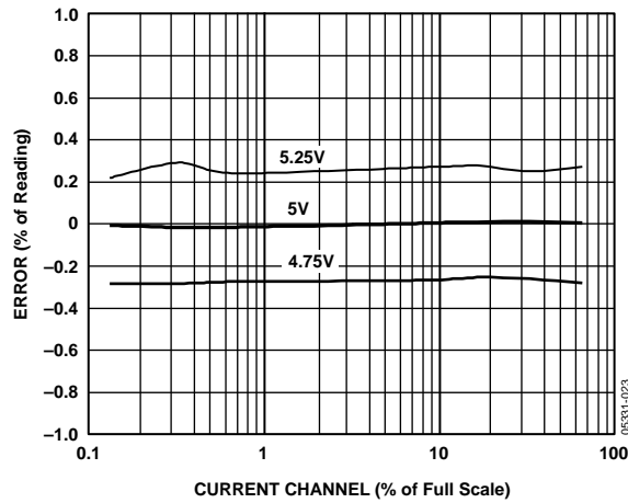
Figure 10. PSR with Internal Reference, PF = 1
