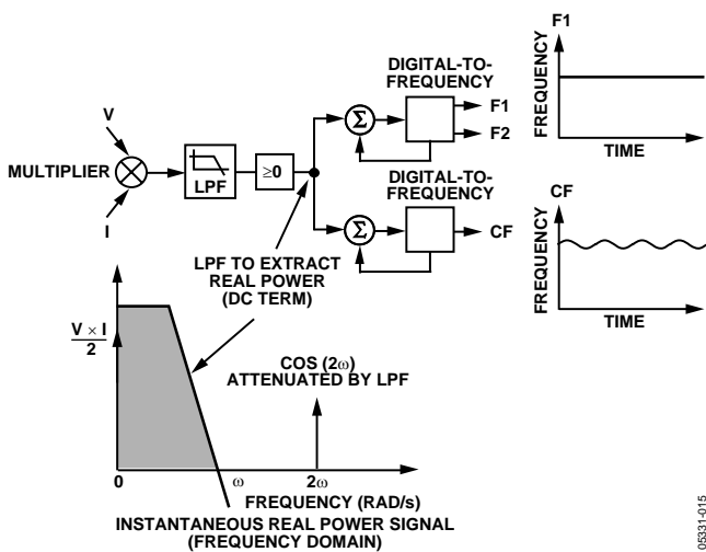
Figure 25. Positive Only Real Power-to-Frequency Conversion
