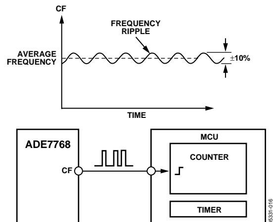
Figure 26. Interfacing the ADE7768 to an MCU
