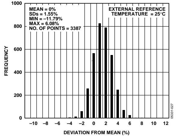
Figure 14. Part-to-Part CF Distribution from Mean
