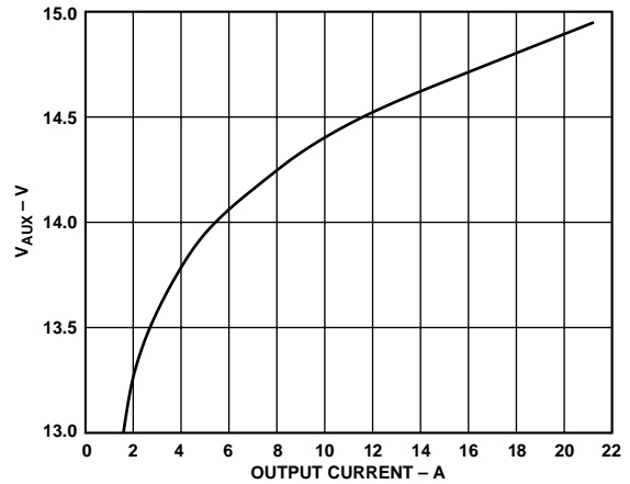
Figure 29. V_{AUX} vs. Converter Output Current (ADDCC02805SA)
