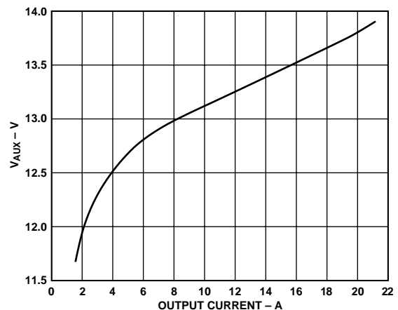
Figure 30. V_{AUX} vs. Converter Output Current (ADDCC02803SC)
