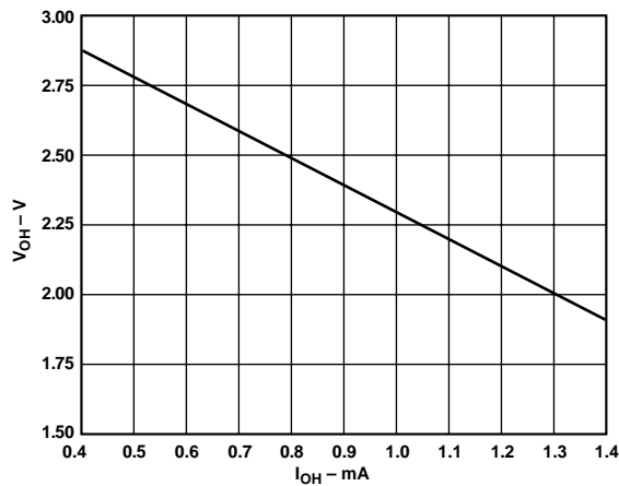
Figure 26. Source Capability of Status Output (ADDCC02803SC)
