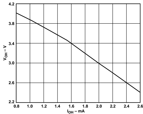
Figure 27. Source Capability of Status Output (ADDCC02805SA)
