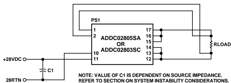
Figure 36. Typical Power Connections and External Parts for Converter
