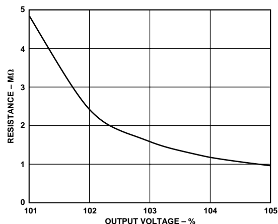
Figure 25. External Resistor for Increasing Output Voltage
