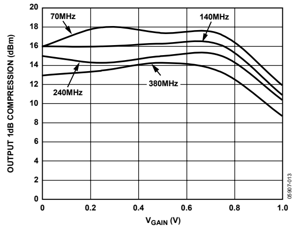
Figure 13. Output Compression Point vs. V_{GAIN} ( V_{MODE} = 0 V )
