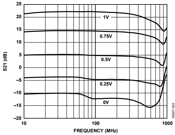
Figure 3. Frequency Response vs. V_{GAIN}
